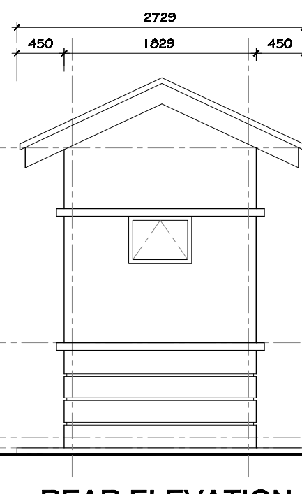
REAR ELEVATION scale 1:50
