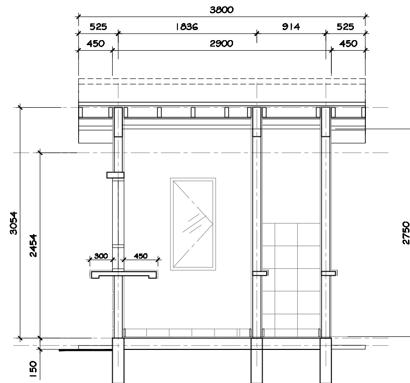
SECTION X-X scale 1:50
