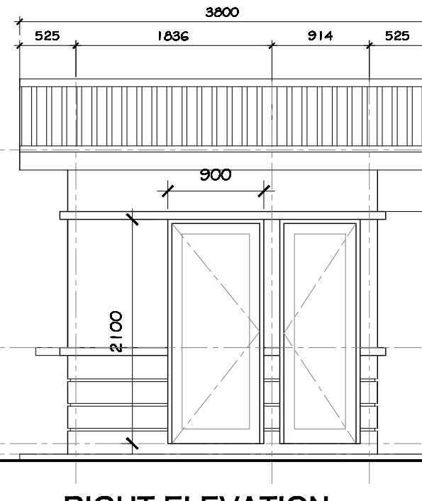
RIGHT ELEVATION scale 1:50
