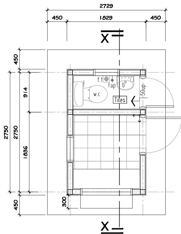
FLOOR PLAN scale 1:50
