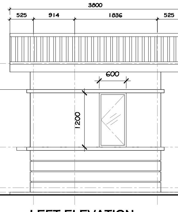
LEFT ELEVATION scale 1:50
