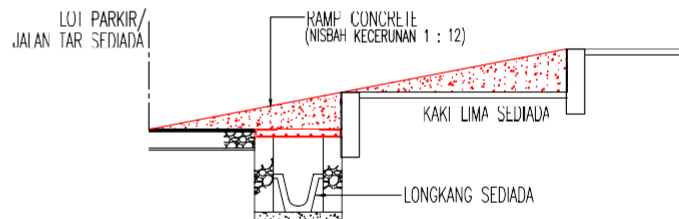
KERATAN LONGKANG CONCRETE
