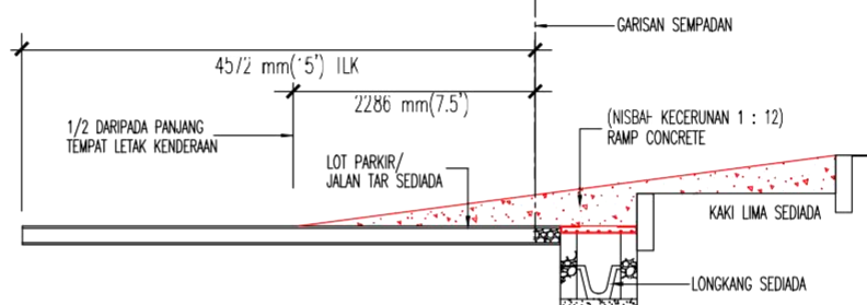
KERATAN LONGKANG CONCRETE
