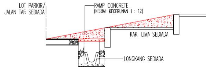
KERAJIAN LONGKANG CONCRETE
